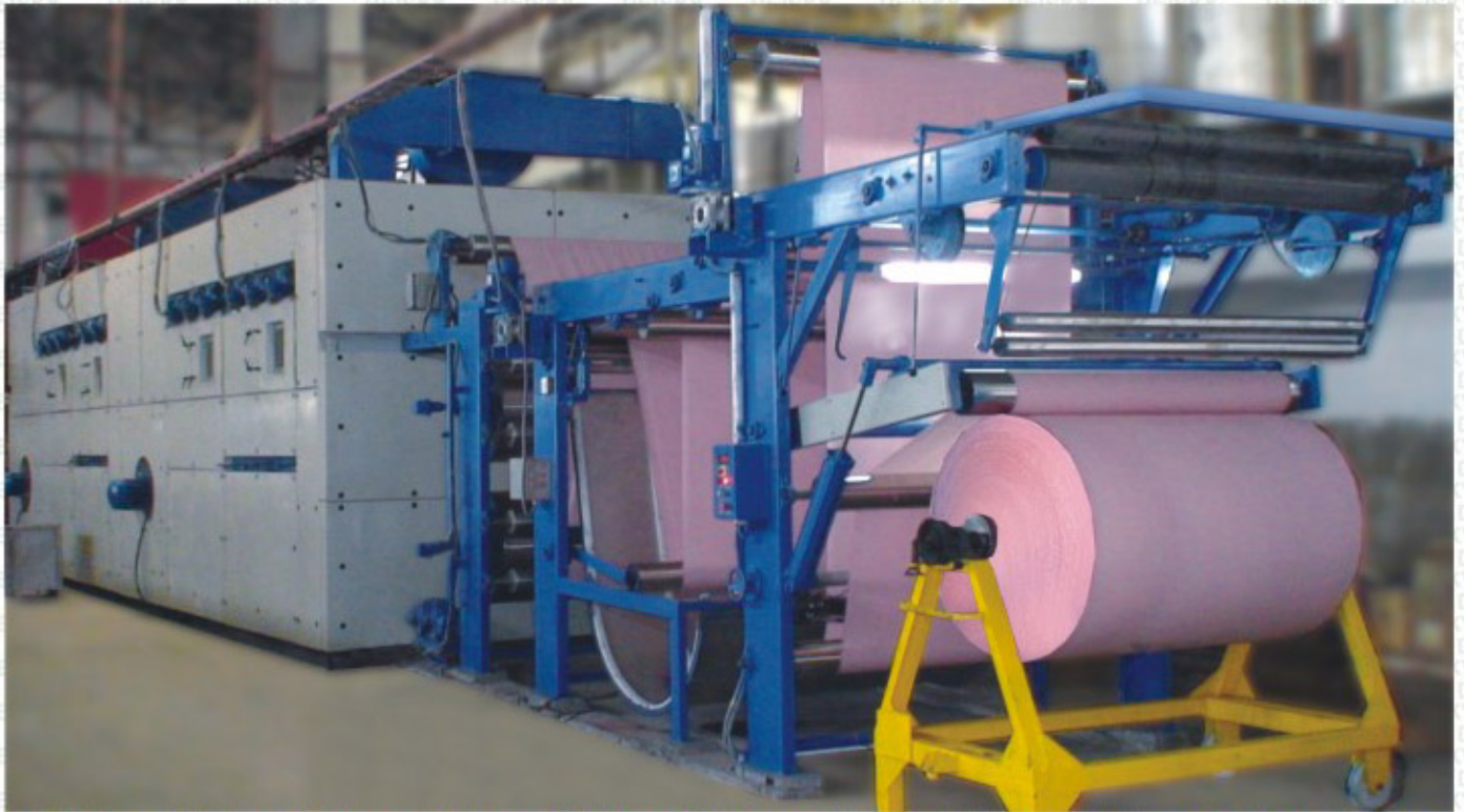
HOT FLUE DRIER WITH "PLEVA" MOISTURE CONTROLLER FOR REACTIVE DYEING
