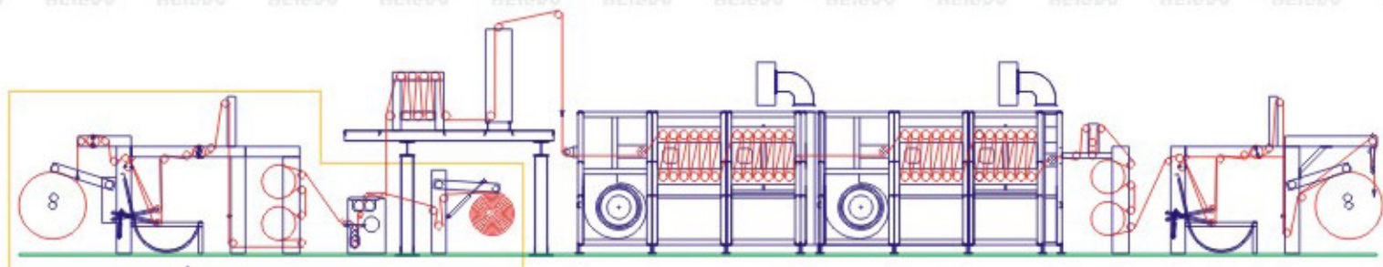
Cold Pad Batch Dyeing
